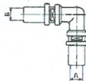
4052 Raccordo gomito femmina. Female elbow fitting.
